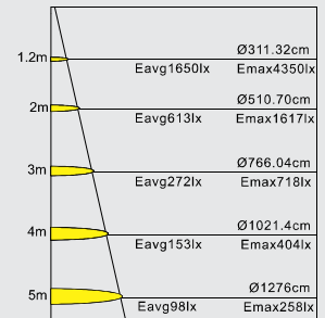
Average illumination intensity diagram
